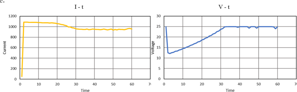
Fig. 7. Current and Voltage Graph Against Time in Photovoltaic Based on P&amp;O Algorithm
