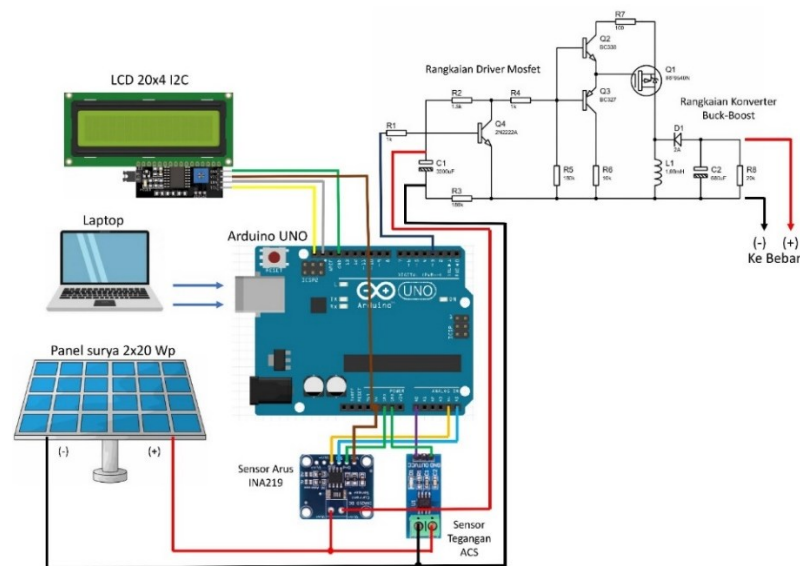
Fig. 3. Overall Circuit
