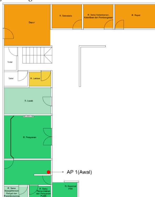
Fig. 3. Visualization of Heatmap AP-1 (Initial) on Floor 1
