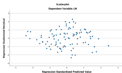
Figure 1. Heteroscedasticity Test
